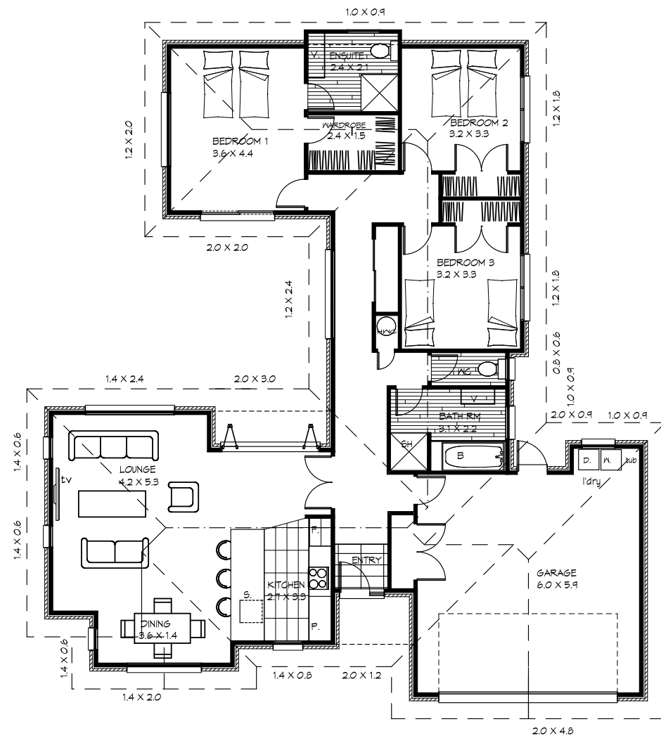
FLOOR PLAN
