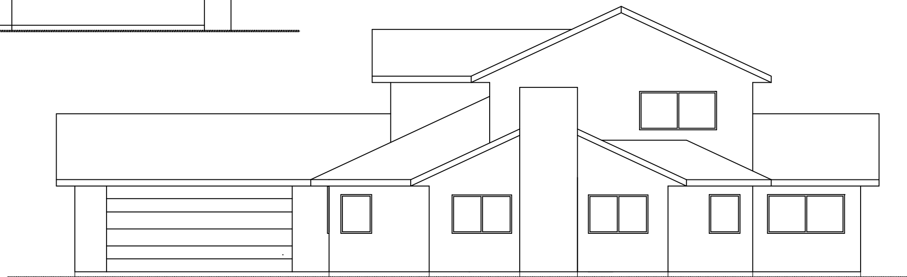
NORTH ELEVATION 1*100
