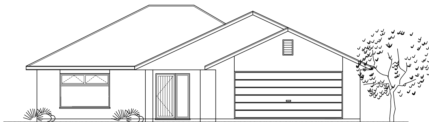
FRONT ELEVATION
