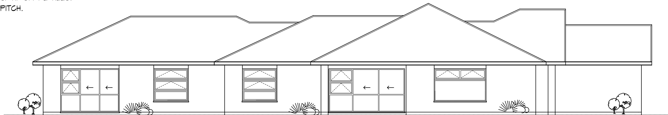
SIDE ELEVATION
