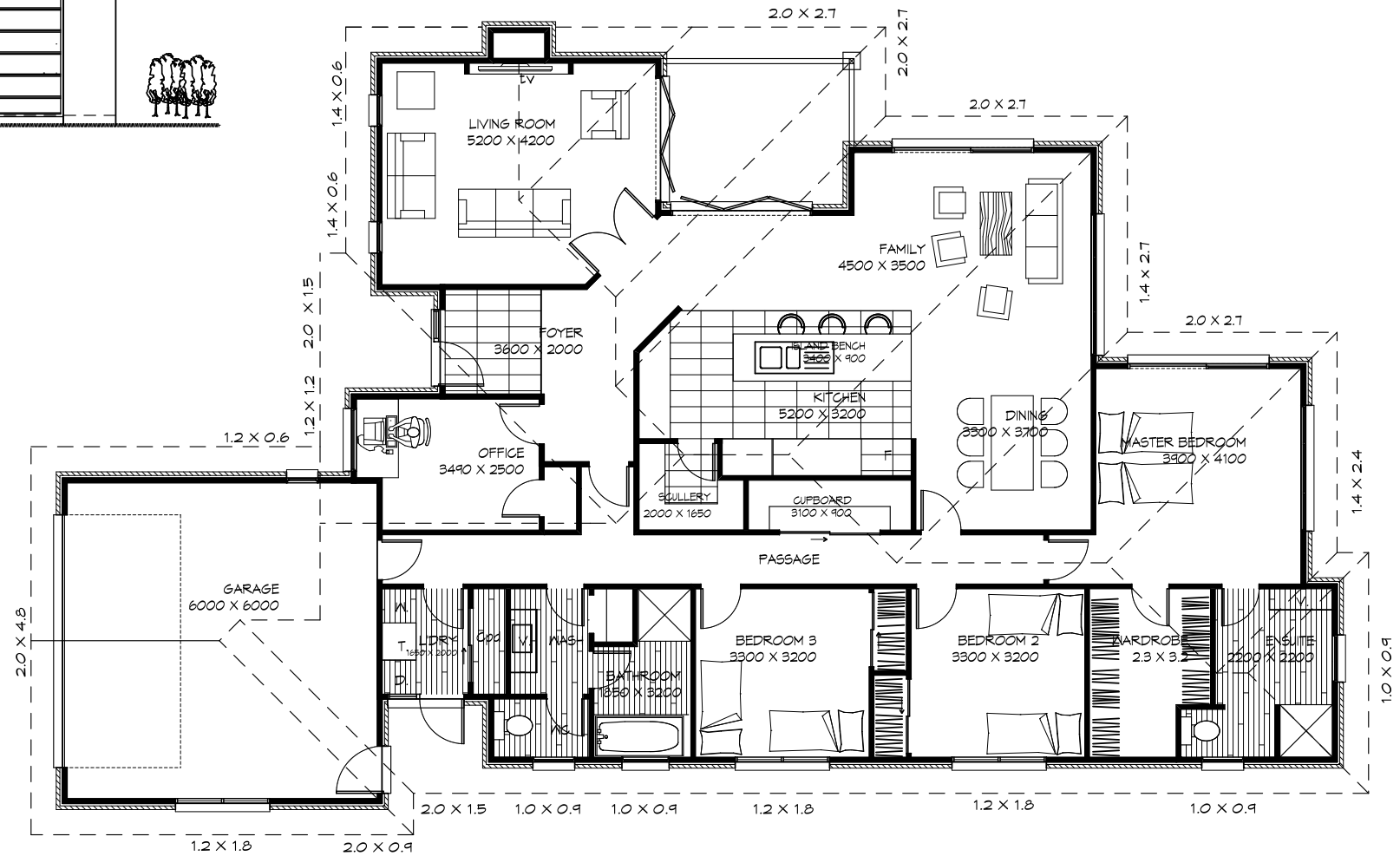
FLOOR PLAN
