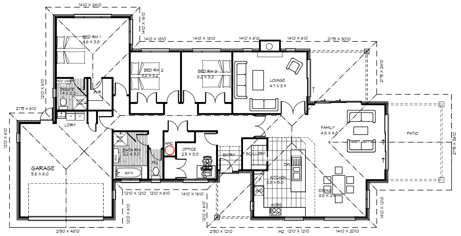
FLOOR PLAN 1:100
